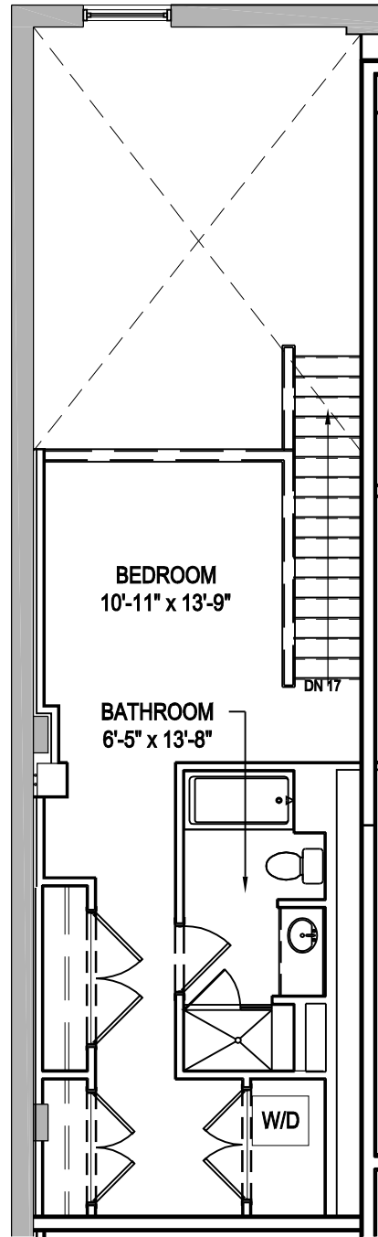
FIFTH FLOOR
